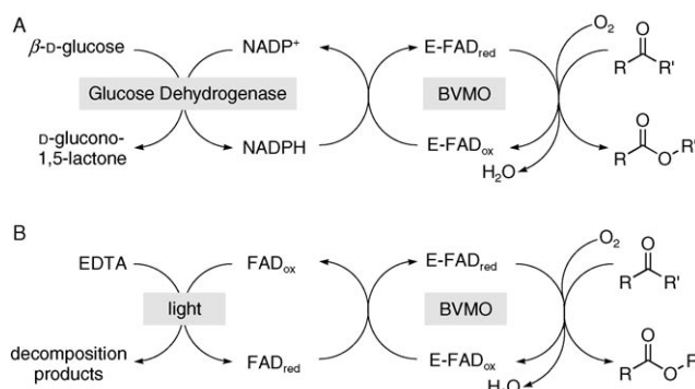
Scheme 1. Comparison of the conventional regeneration of a Baeyer–Villiger monooxygenase (BVMO, e.g. PAMO) for catalysis through enzymatic regeneration of NADPH (A) and the novel simplified light-driven pathway using a flavin (B). Part (A) shows an enzyme-coupled regeneration system employing the common glucose dehydrogenase to catalyze the regeneration of the reduced nicotinamide cofactor. The use of this coupled enzyme can be replaced by visible light, which reduces the complexity of the setup by eliminating the need for a coupled enzyme. (E-FAD: enzyme bound flavin adenine dinucleotide.)
