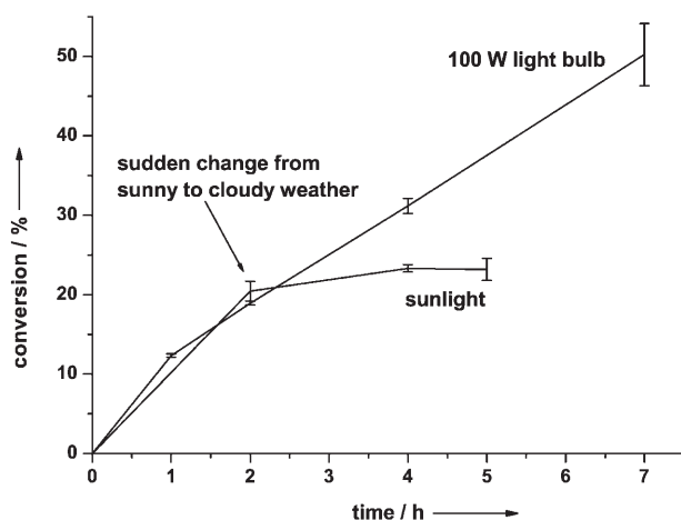
Figure 1. Time-resolved conversion of the light-driven BV reaction of rac - 1a . Conditions for sunlight-driven reactions: 10 \mu\text{M} PAMO P3, 25 mM EDTA, 100 \mu\text{M} FAD, 250 \mu\text{M} NADP + , 1 mM substrate, 50 mM Tris (pH 7.4). Reaction vessels were placed on aluminum foil and exposed to sunlight. For comparison, the reaction employing a lamp as light source is also shown.
